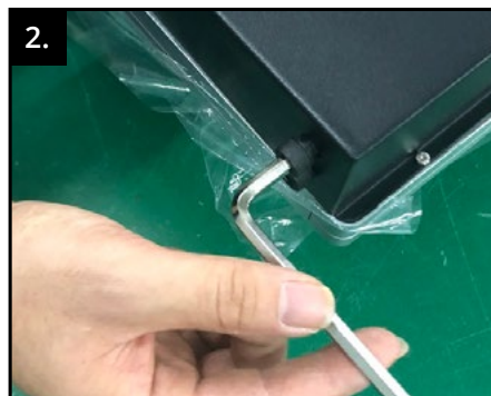
2. Unscrew all allen screws (10 pcs.) from the underside of the display.
